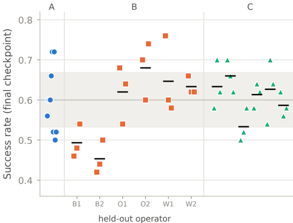
Square, Stage 1: 50 rollouts per checkpoint
