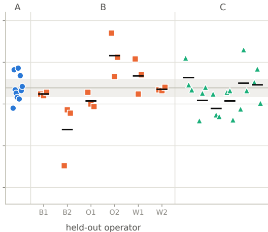
Square, Stage 2: same checkpoints, 500 rollouts
