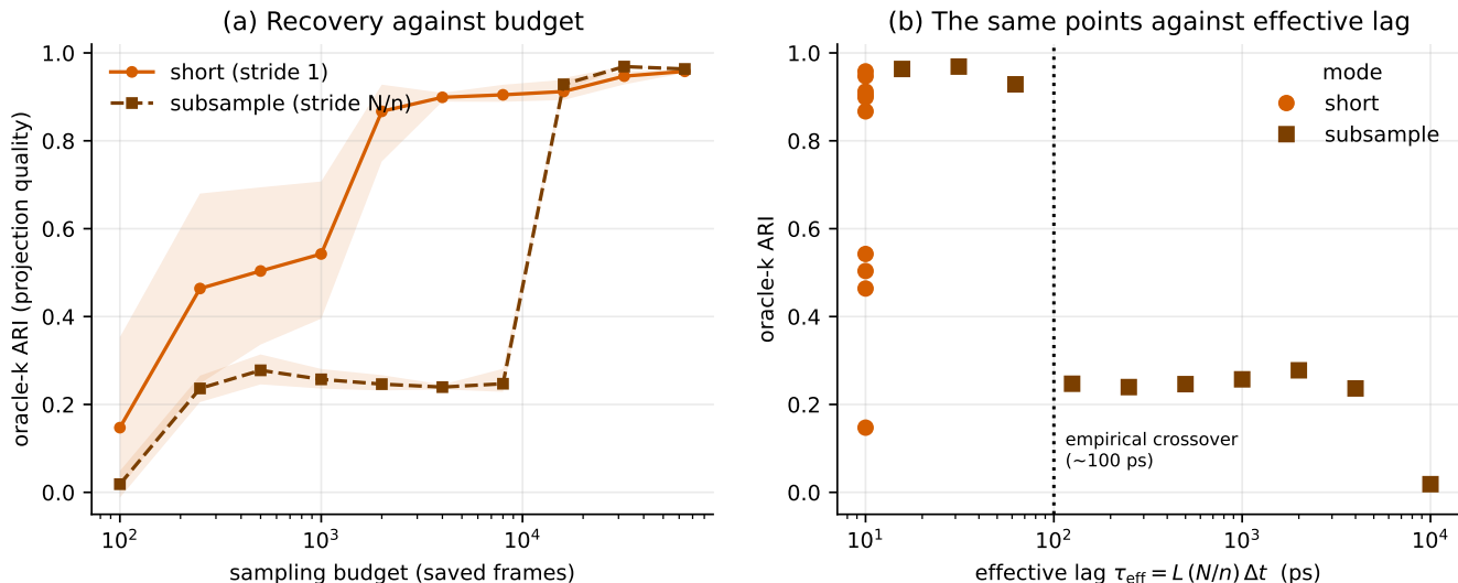
Figure 7: Thinning a trajectory rescales TICA’s lag. (a) Recovery against sampling budget for both modes. (b) The same points against the effective lag \tau_{\text{eff}} = L(N/n)\Delta t : every subsample point above the empirical 100 ps crossover sits near 0.25 and points below it jump to roughly 0.95. This association is descriptive, not a fitted transition timescale. The short points sit at a fixed 10 ps and still span 0.15 to 0.96, so their spread is sample size alone.
