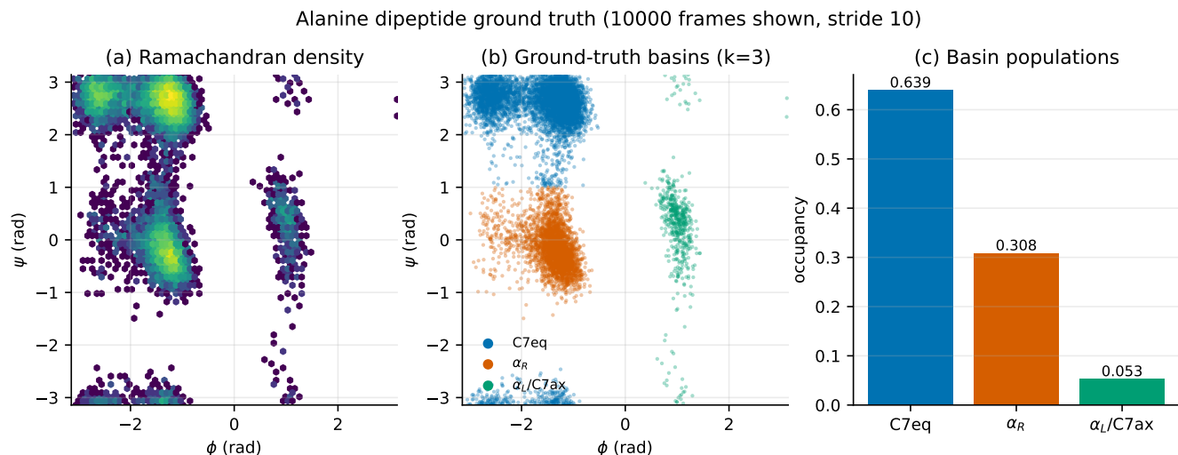
Figure 8: Alanine dipeptide ground truth, from the seed-1 trajectory: (a) Ramachandran density, (b) the standard three-region partition that supplies the basin labels, (c) basin occupancy. The partition is a chemical definition and is independent of every method under audit. The rarest basin holds 5.3% of frames, which is why sampling budget bites hardest on this system.
