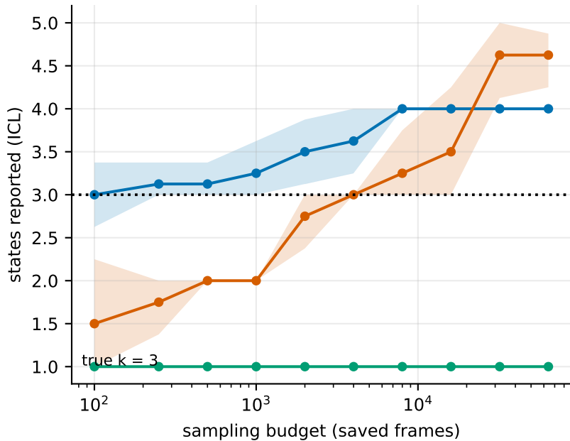
short trajectories
