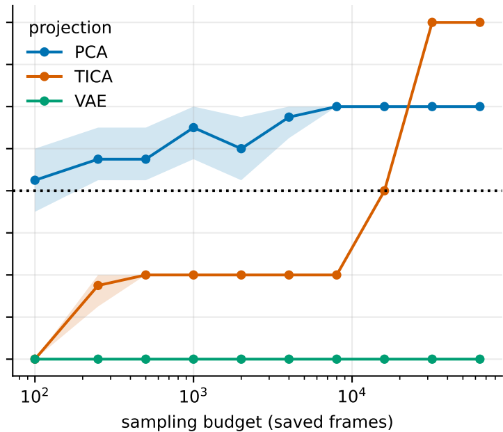
coverage-matched subsample
