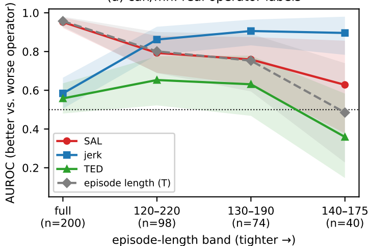
(a) can/mh: real operator labels
