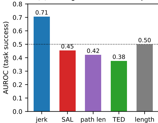
(b) can/mg: T fixed at 150 steps
