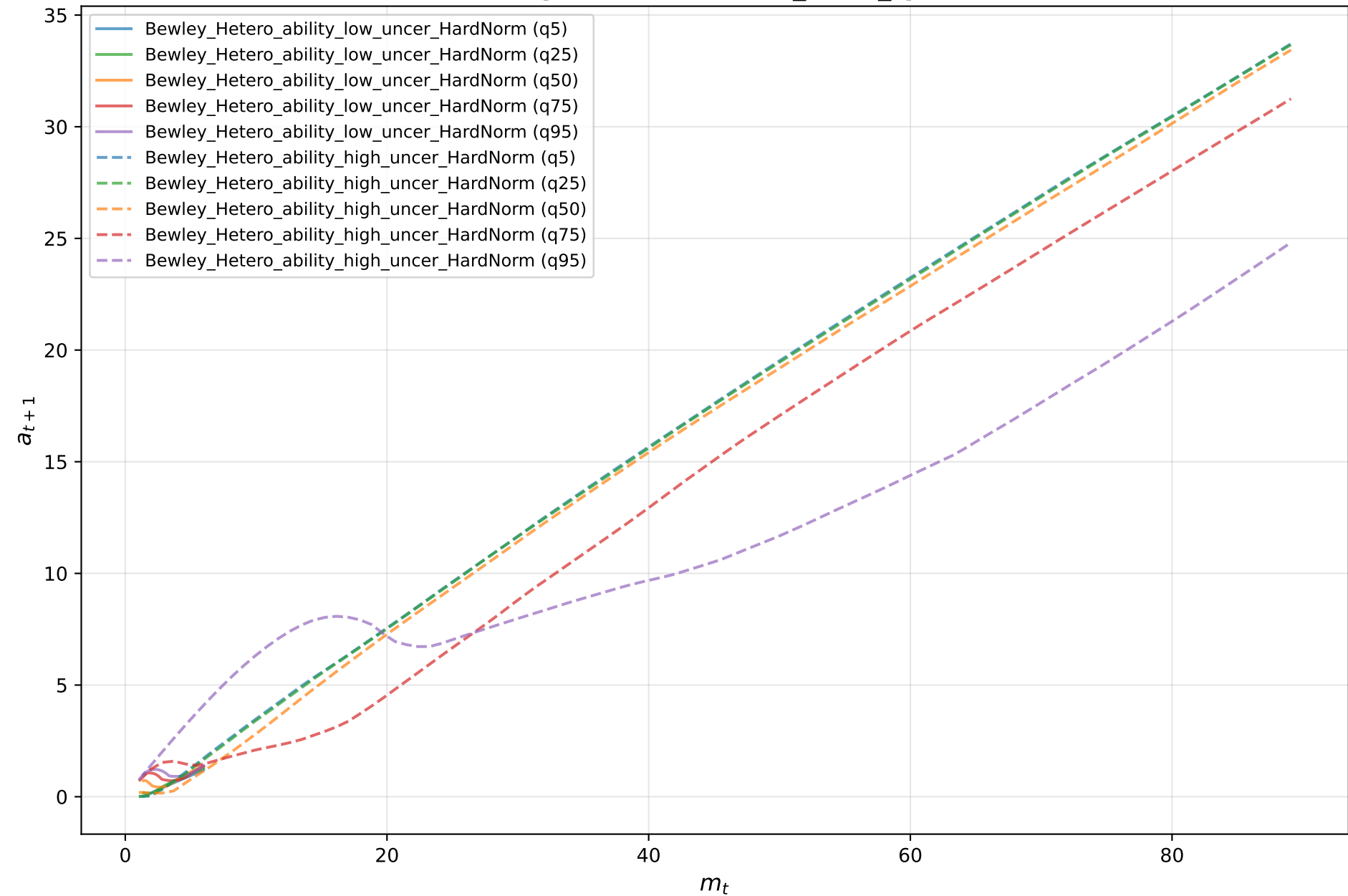
Comparison: A1-1 ( m_t \rightarrow a_{tp1} )
