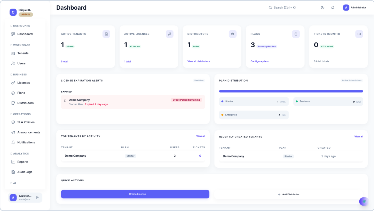
Figure 3: Dashboard Overview & Real-Time Telemetry
