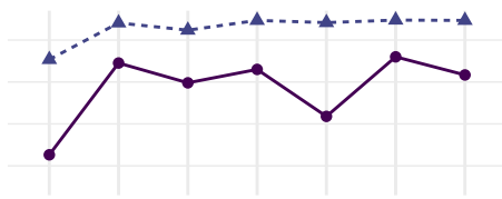
4 -Class Model
