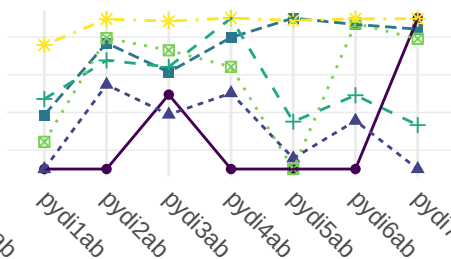
6 -Class Model
