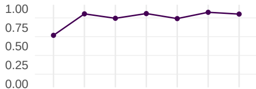
3 -Class Model
