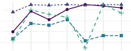
6 -Class Model
