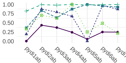
5 -Class Model
