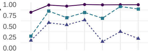
5 -Class Model
