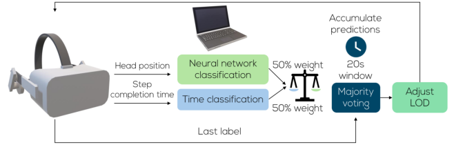
Figure 2: AR application: Data from the headset is streamed to the PC, where NN classification is combined with temporal thresholding and accumulated for 20 seconds, to inform the LOD adjustment.
