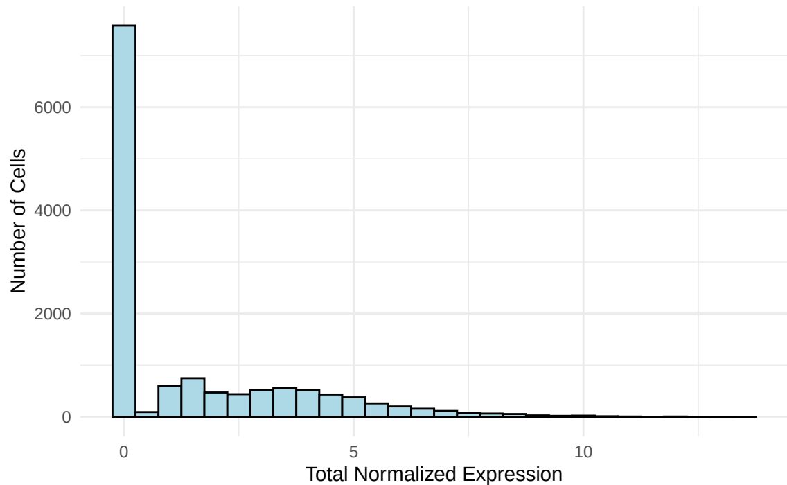
Total Normalized Light Chain Expression per Cell
