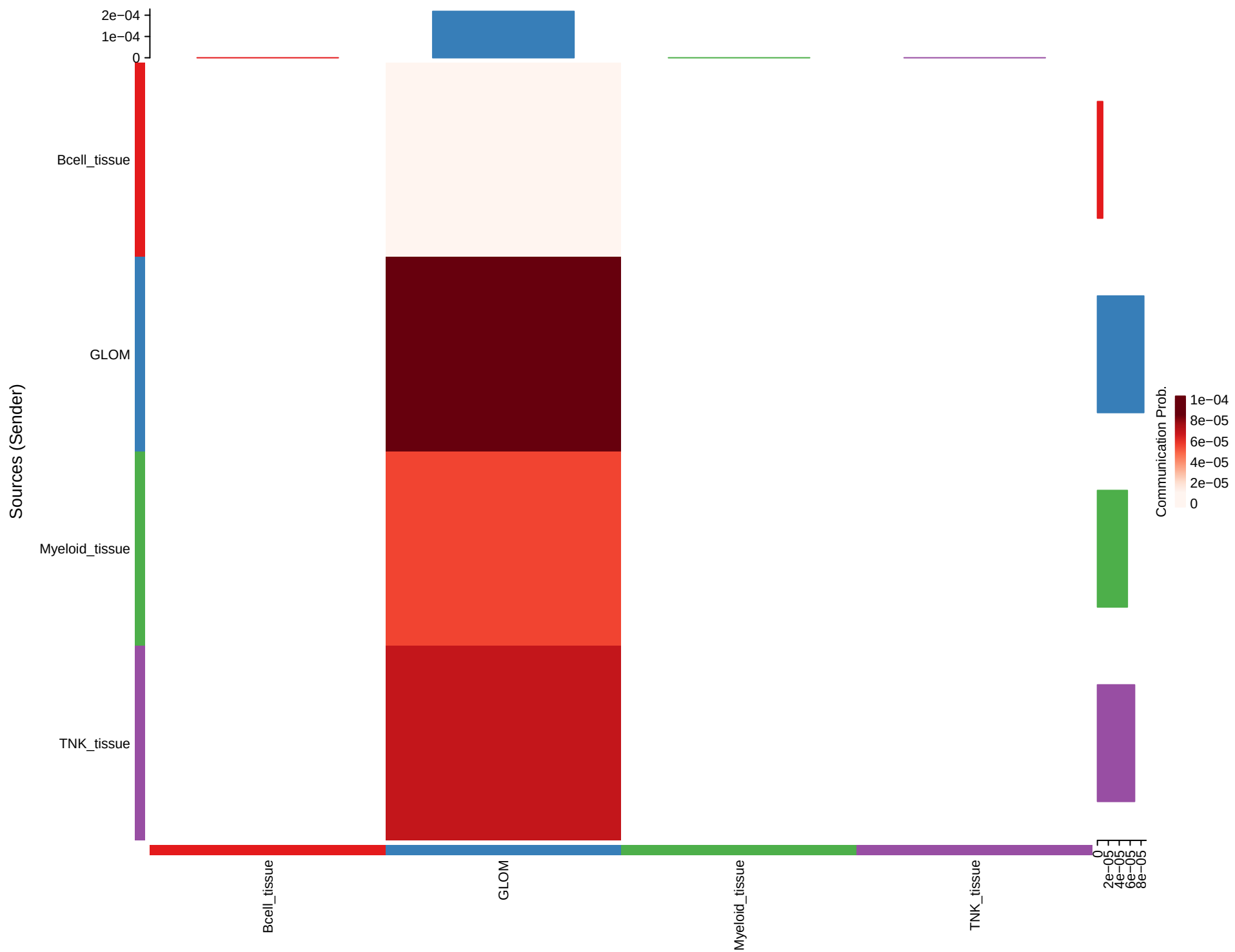
CD46 signaling network
