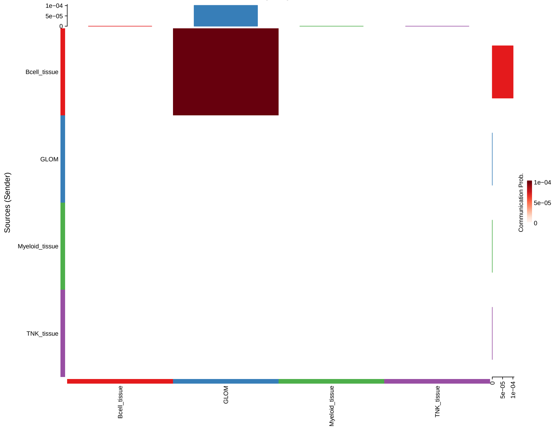
SELL signaling network
