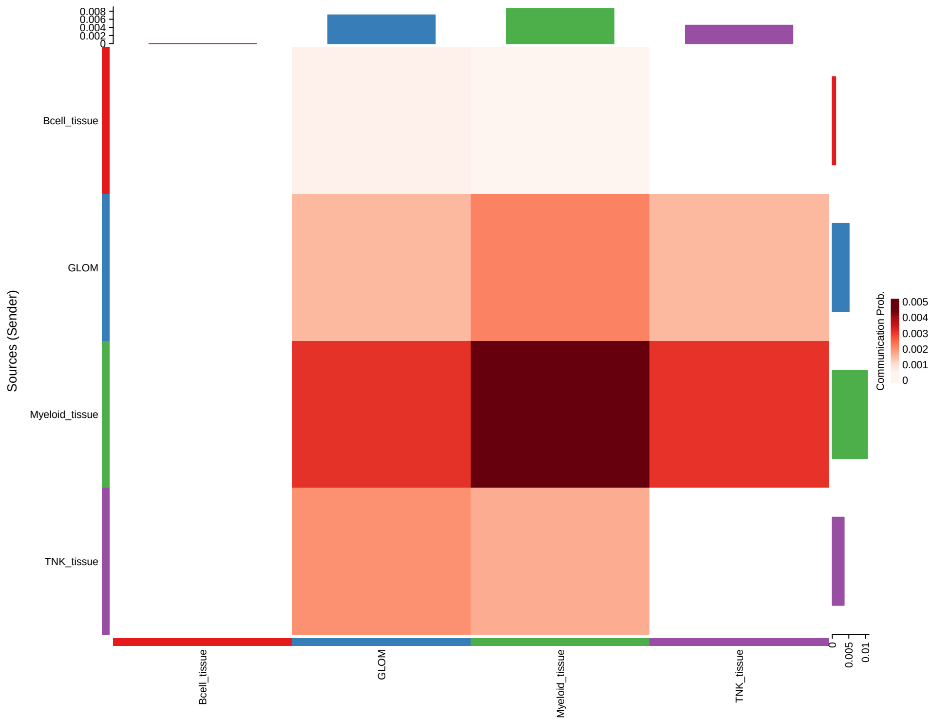
SPP1 signaling network
