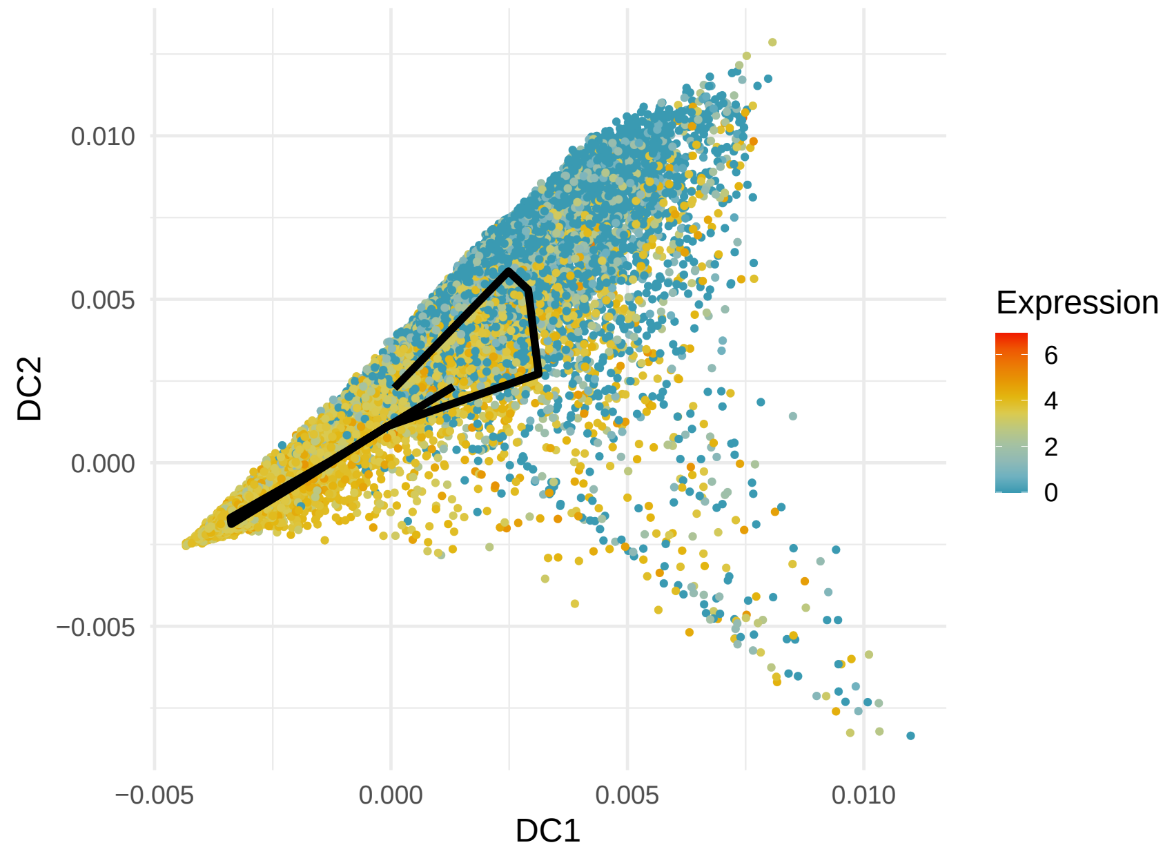
IGHM Expression along Lineage 1 ( R = -0.254 )
