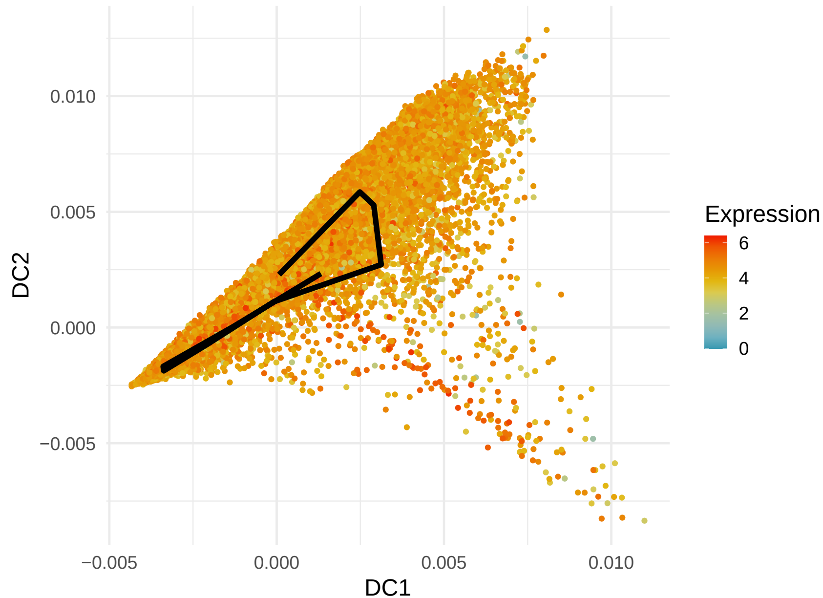
MT-ATP6 Expression along Lineage 1 ( R = -0.215 )
