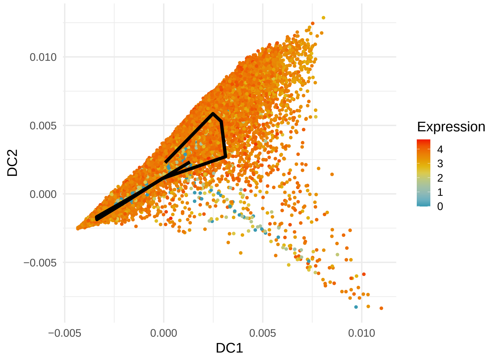
RPL23A Expression along Lineage 1 ( R = 0.465 )
