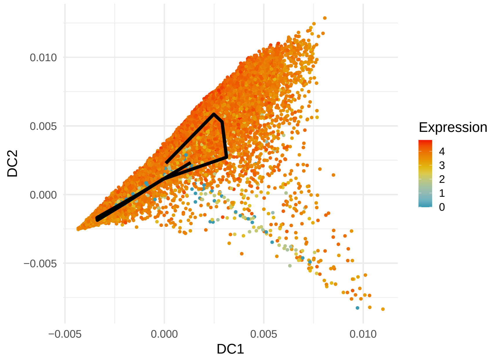
RPS14 Expression along Lineage 1 ( R = 0.502 )
