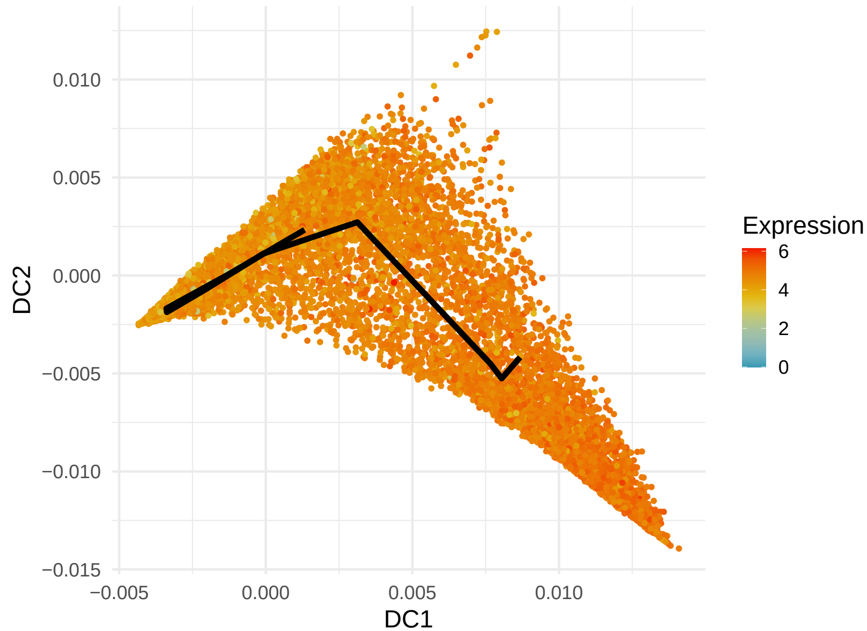
B2M Expression along Lineage 2 (R= 0.404)
