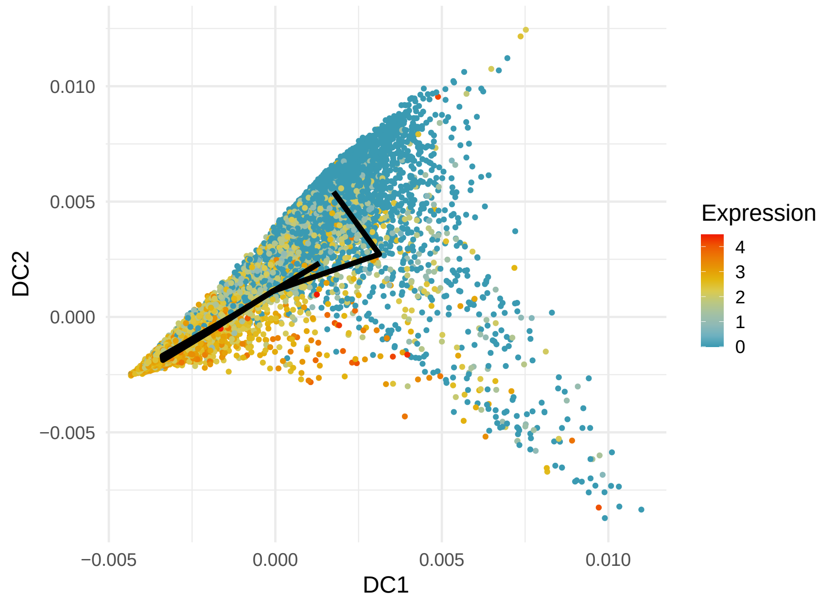
IGHD Expression along Lineage 3 ( R = -0.219 )
