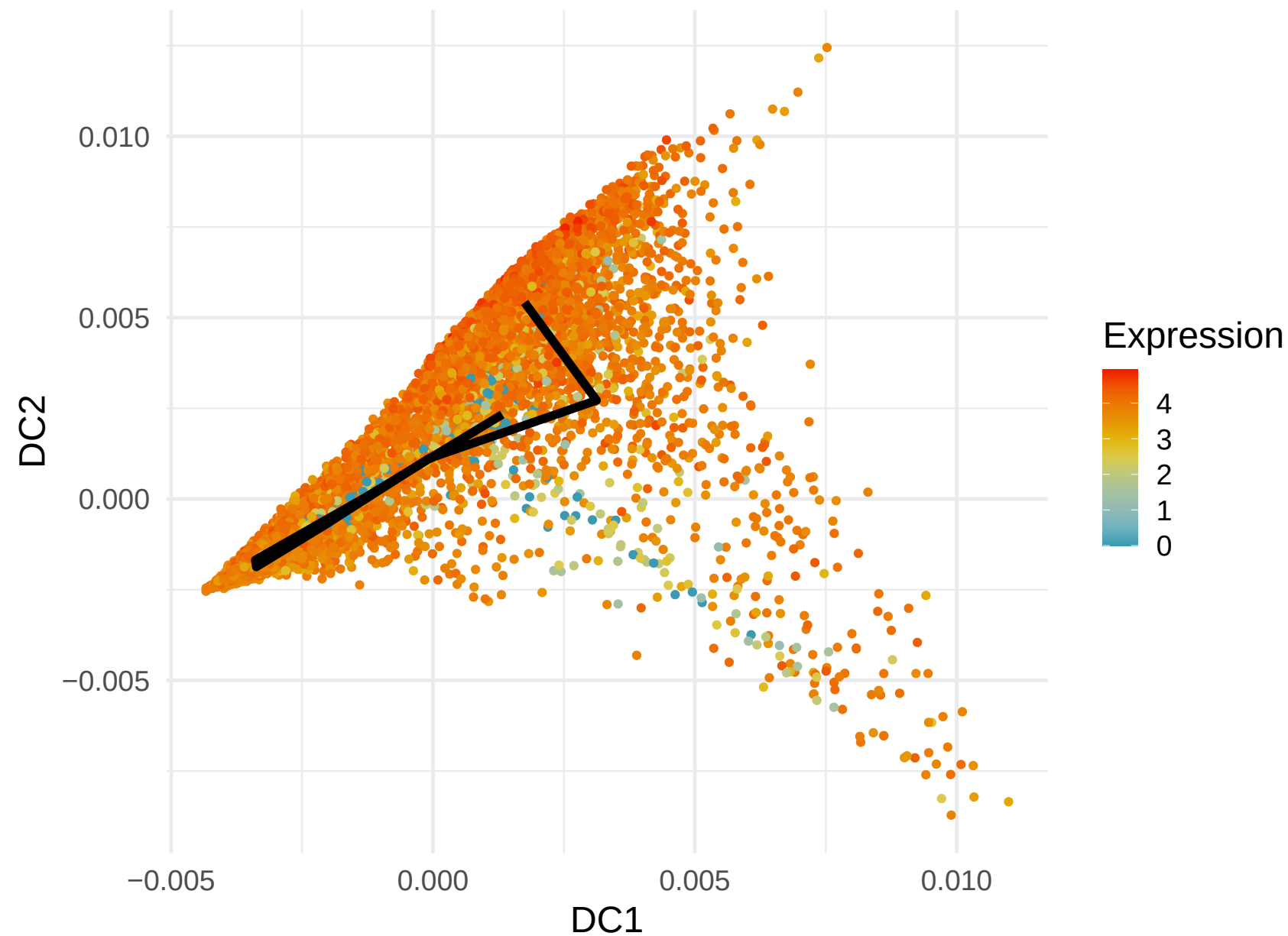
RPS15A Expression along Lineage 3 ( R = 0.519 )
