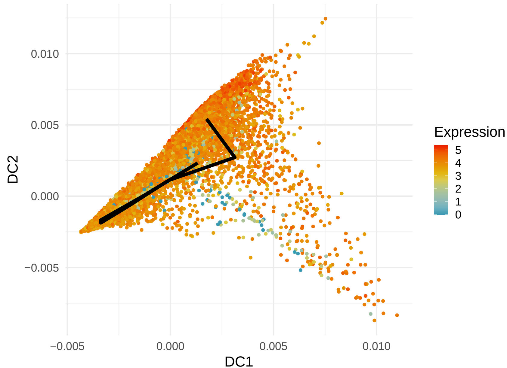
RPS29 Expression along Lineage 3 ( R = 0.542 )
