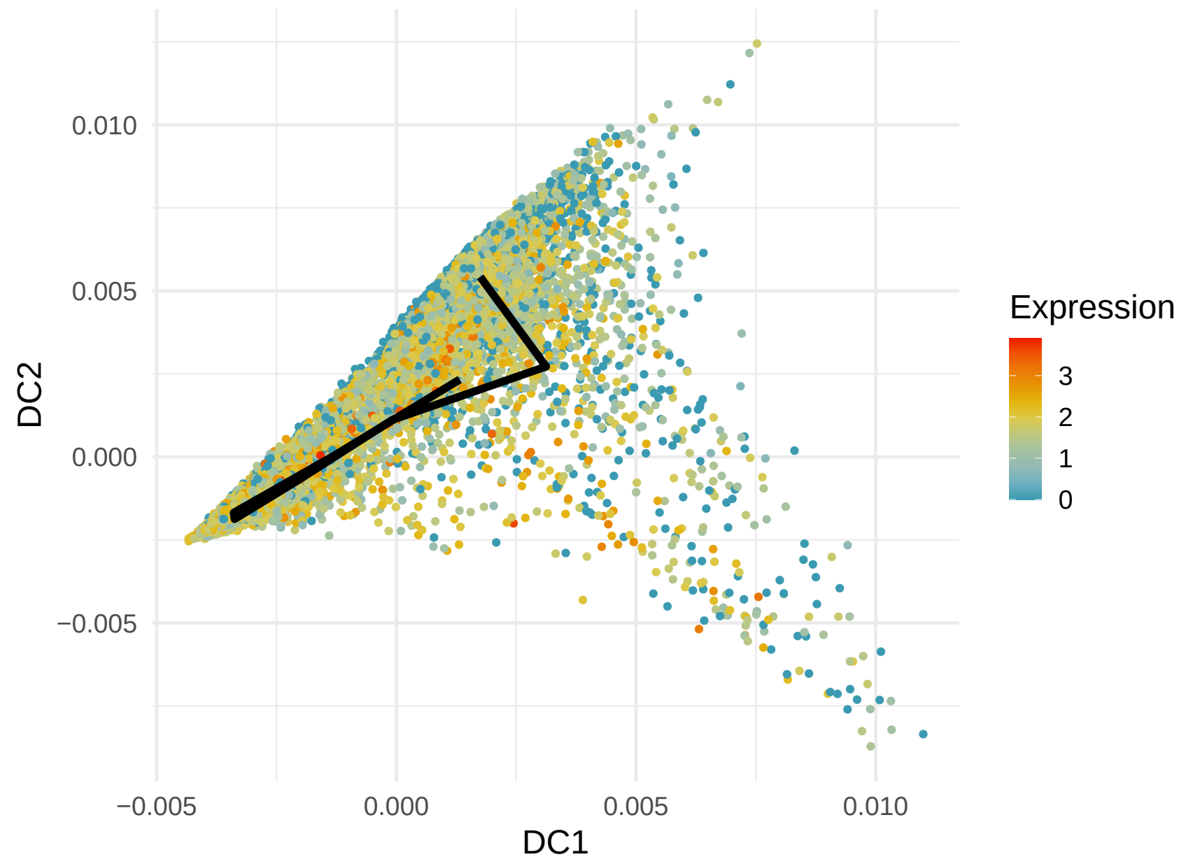
SF1 Expression along Lineage 3 ( R = -0.22 )
