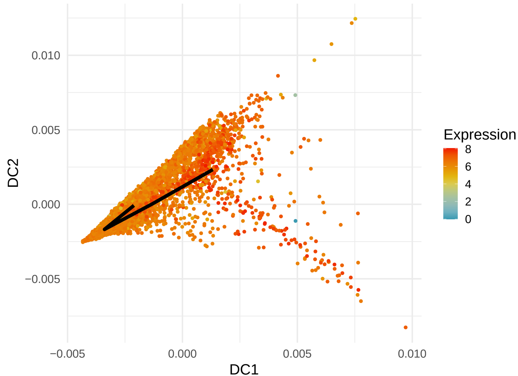
MALAT1 Expression along Lineage 4 ( R = -0.511 )
