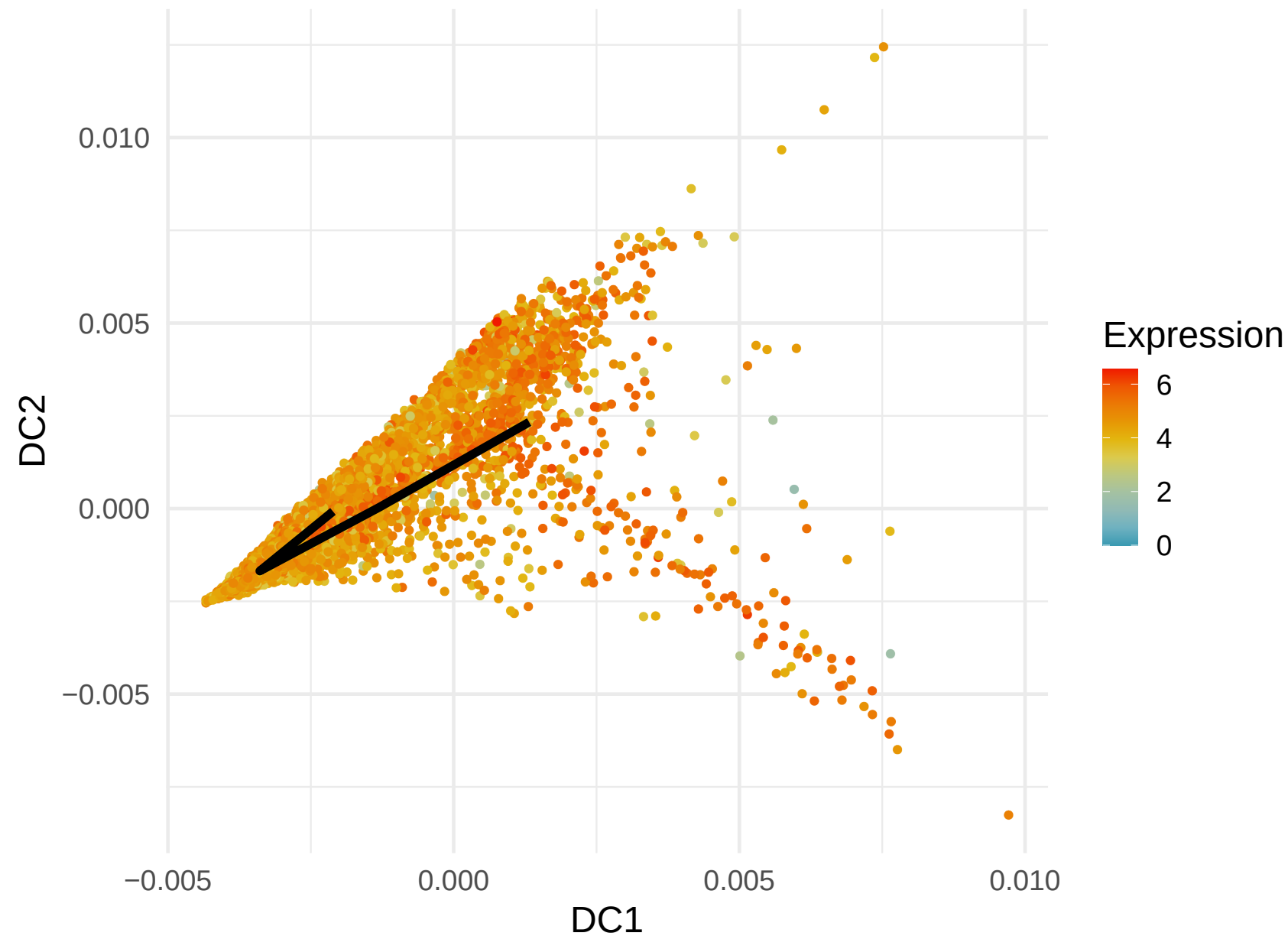
MT-ATP6 Expression along Lineage 4 ( R = -0.208 )
