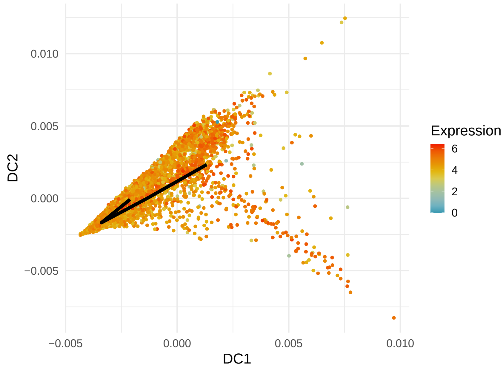
MT-CO3 Expression along Lineage 4 ( R = -0.21 )
