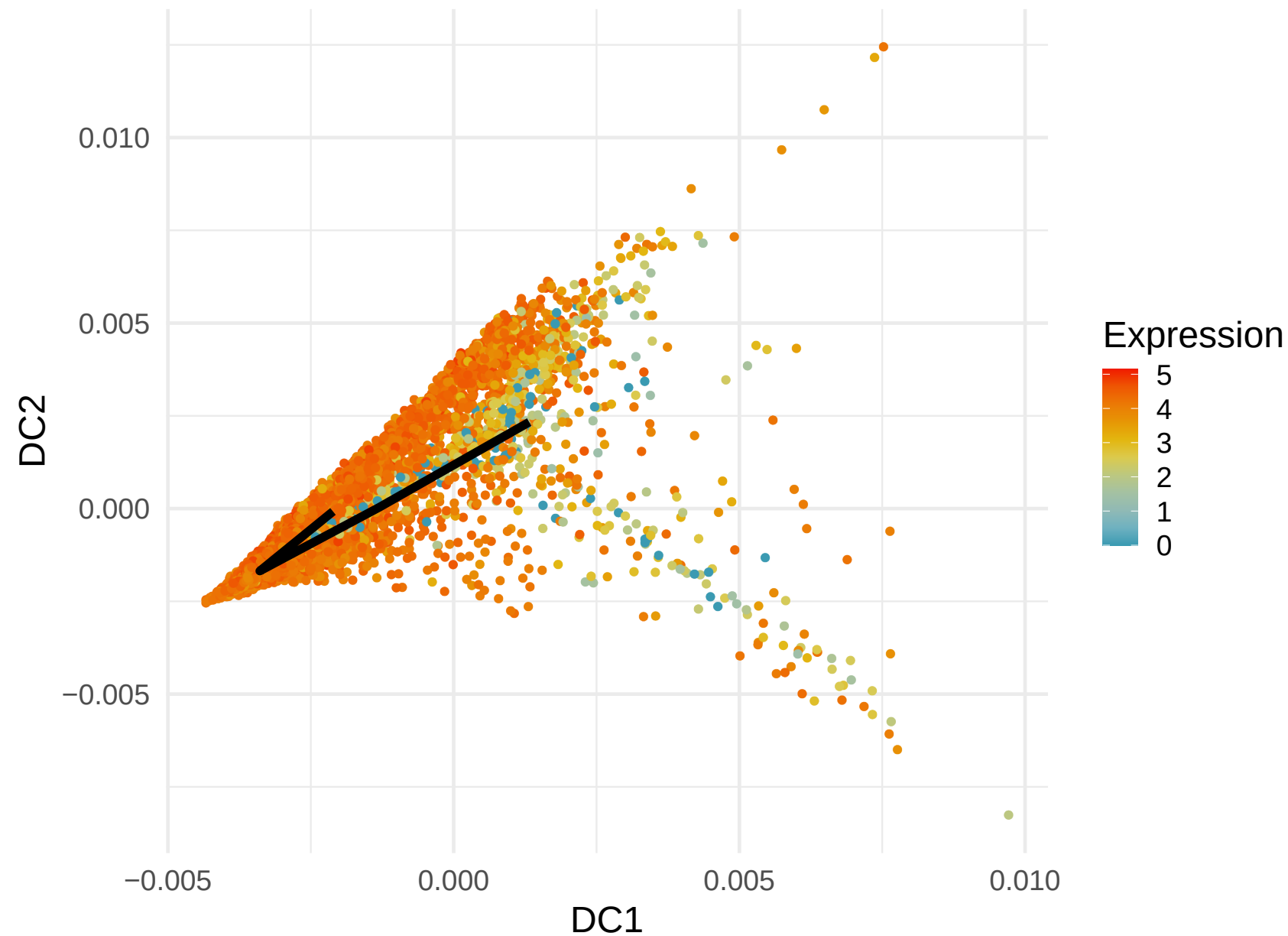
RPL30 Expression along Lineage 4 ( R = 0.603 )
