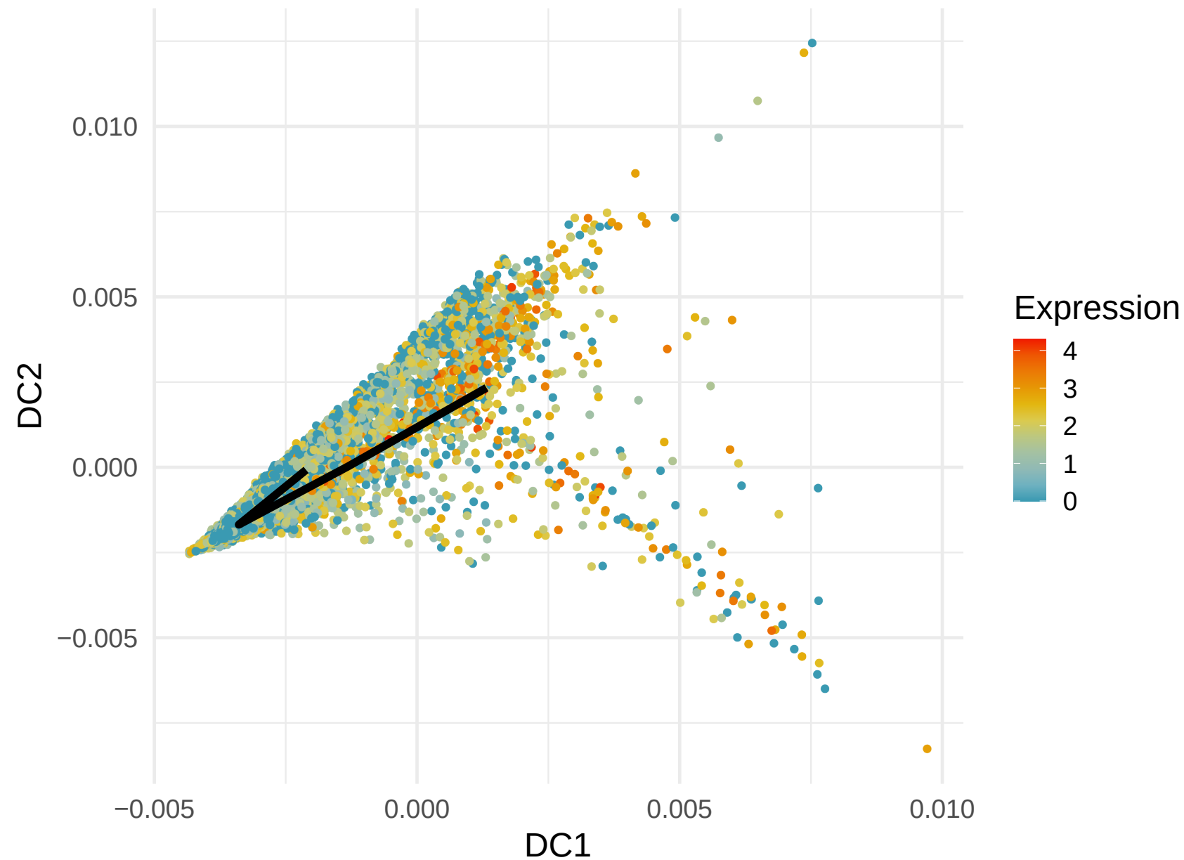
XIST Expression along Lineage 4 ( R = -0.247 )
