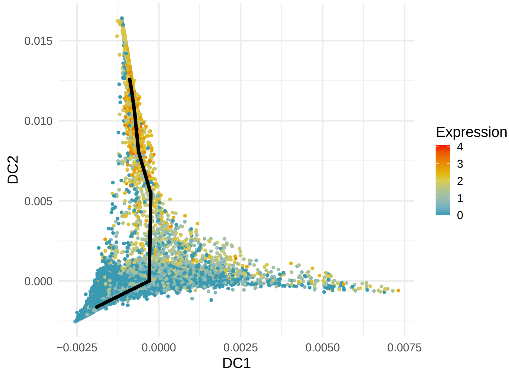
CD81 Expression along Lineage 1 ( R = 0.328 )
