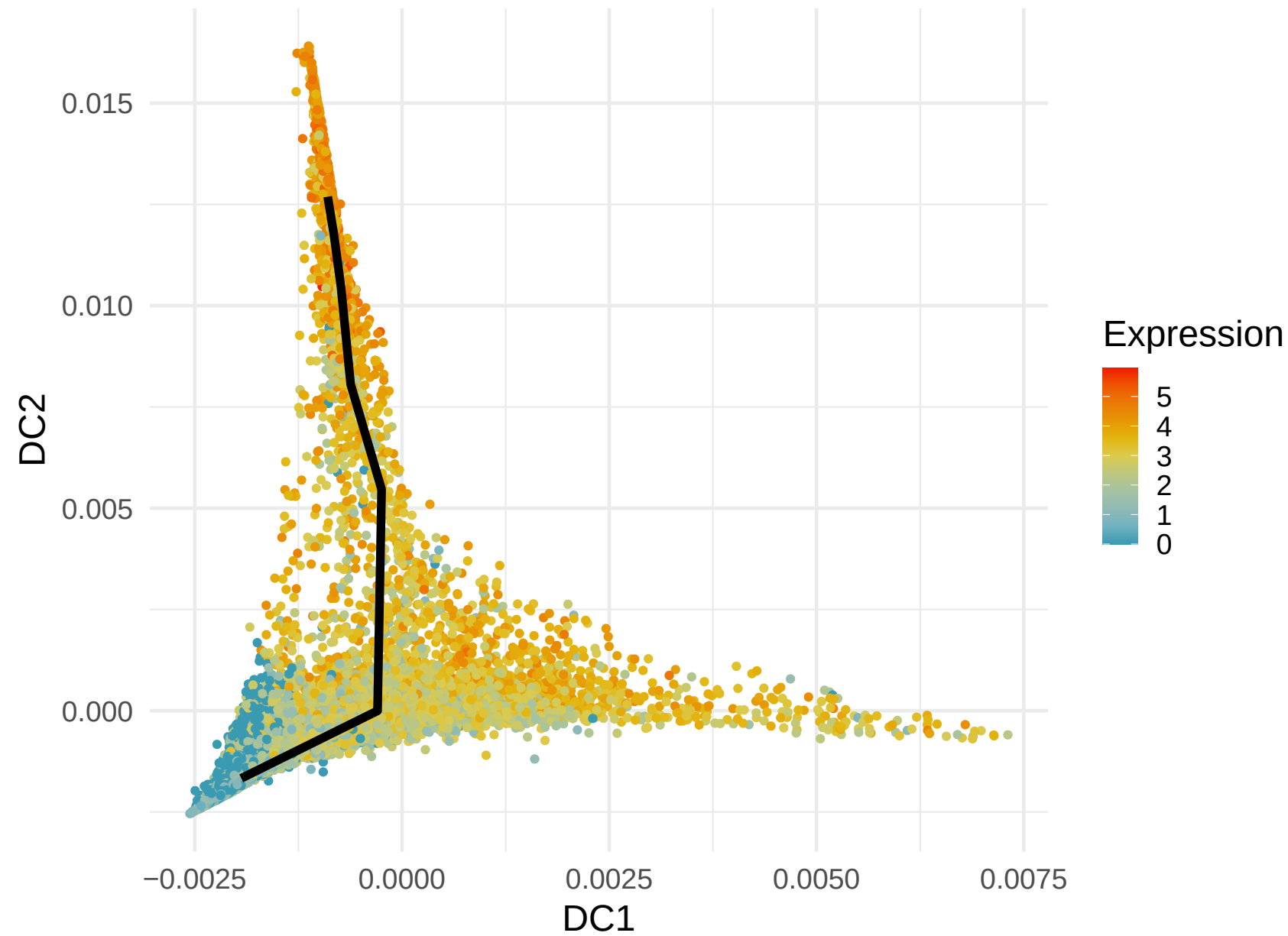
HLA-DRB1 Expression along Lineage 1 ( R = 0.42 )
