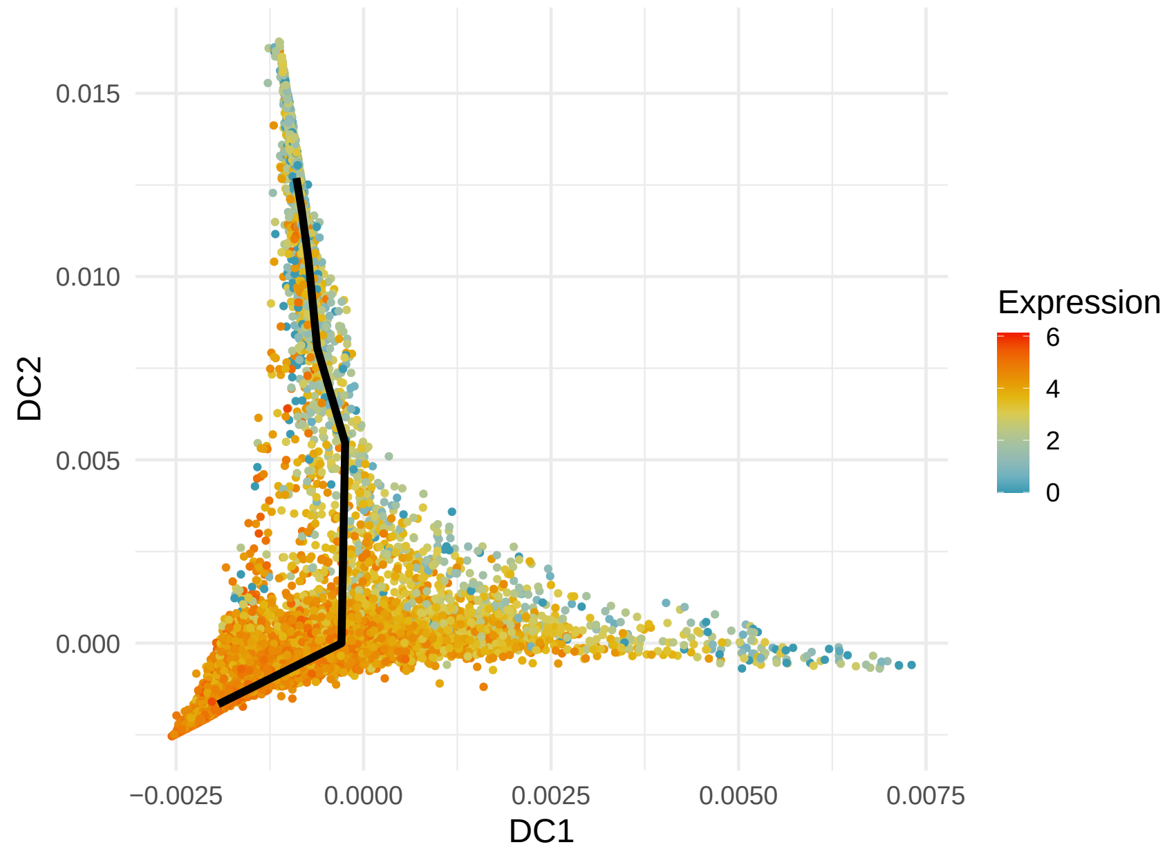
LYZ Expression along Lineage 1 ( R = -0.272 )
