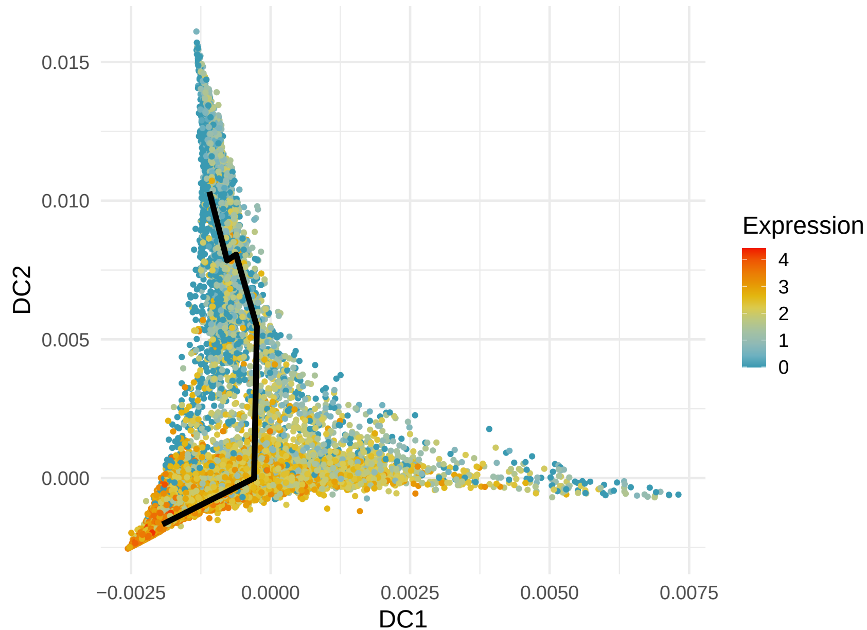
MNDA Expression along Lineage 2 ( R = -0.308 )
