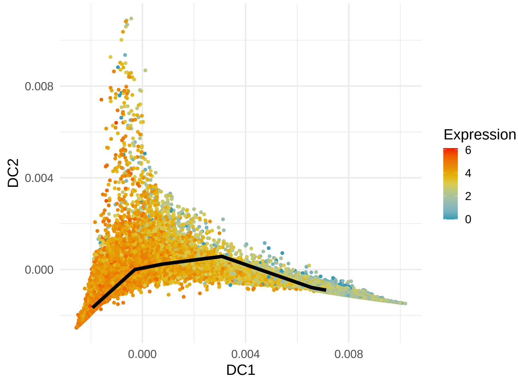
LYZ Expression along Lineage 3 ( R = -0.599 )
