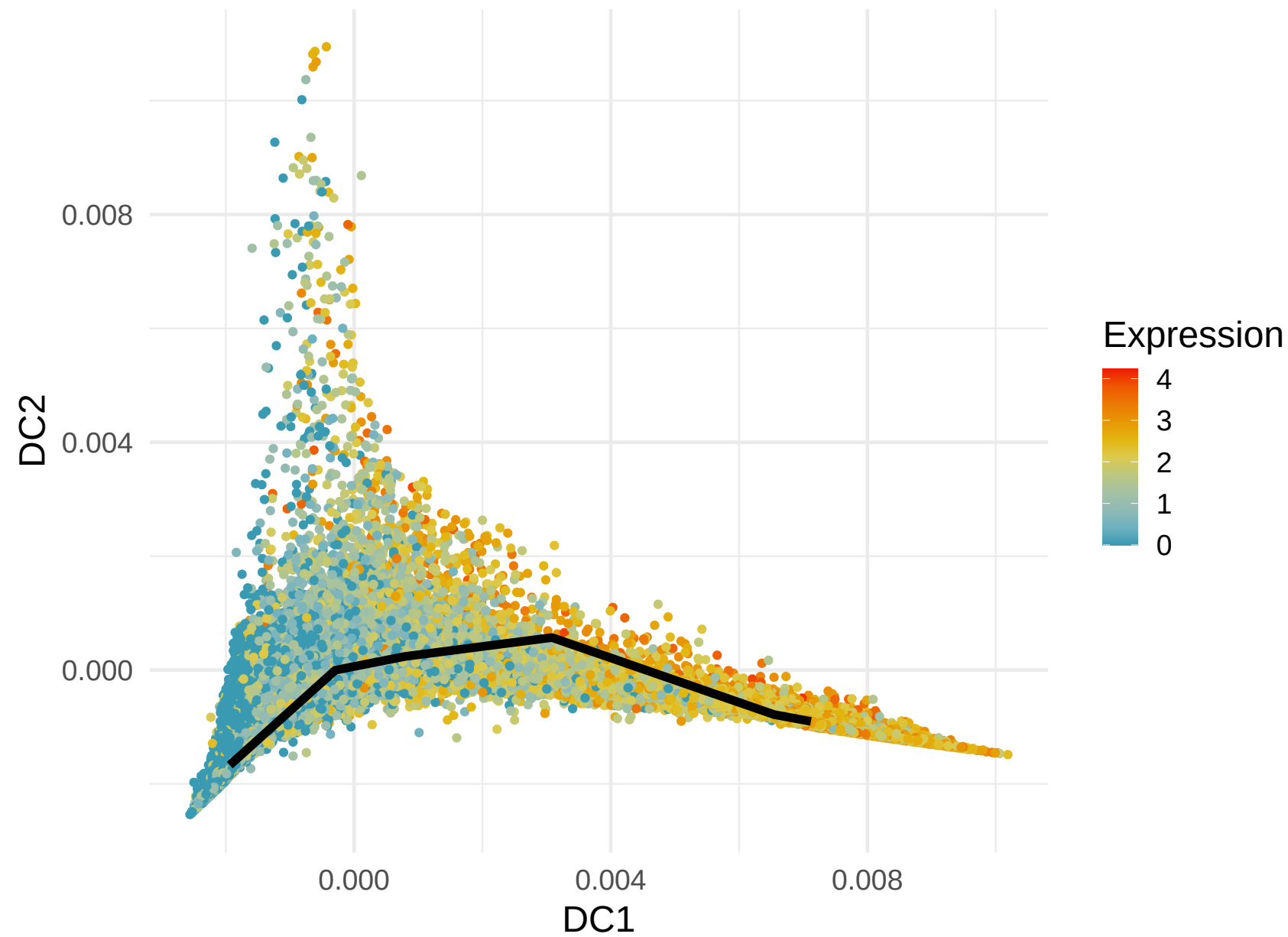
MS4A7 Expression along Lineage 3 (R= 0.547)
