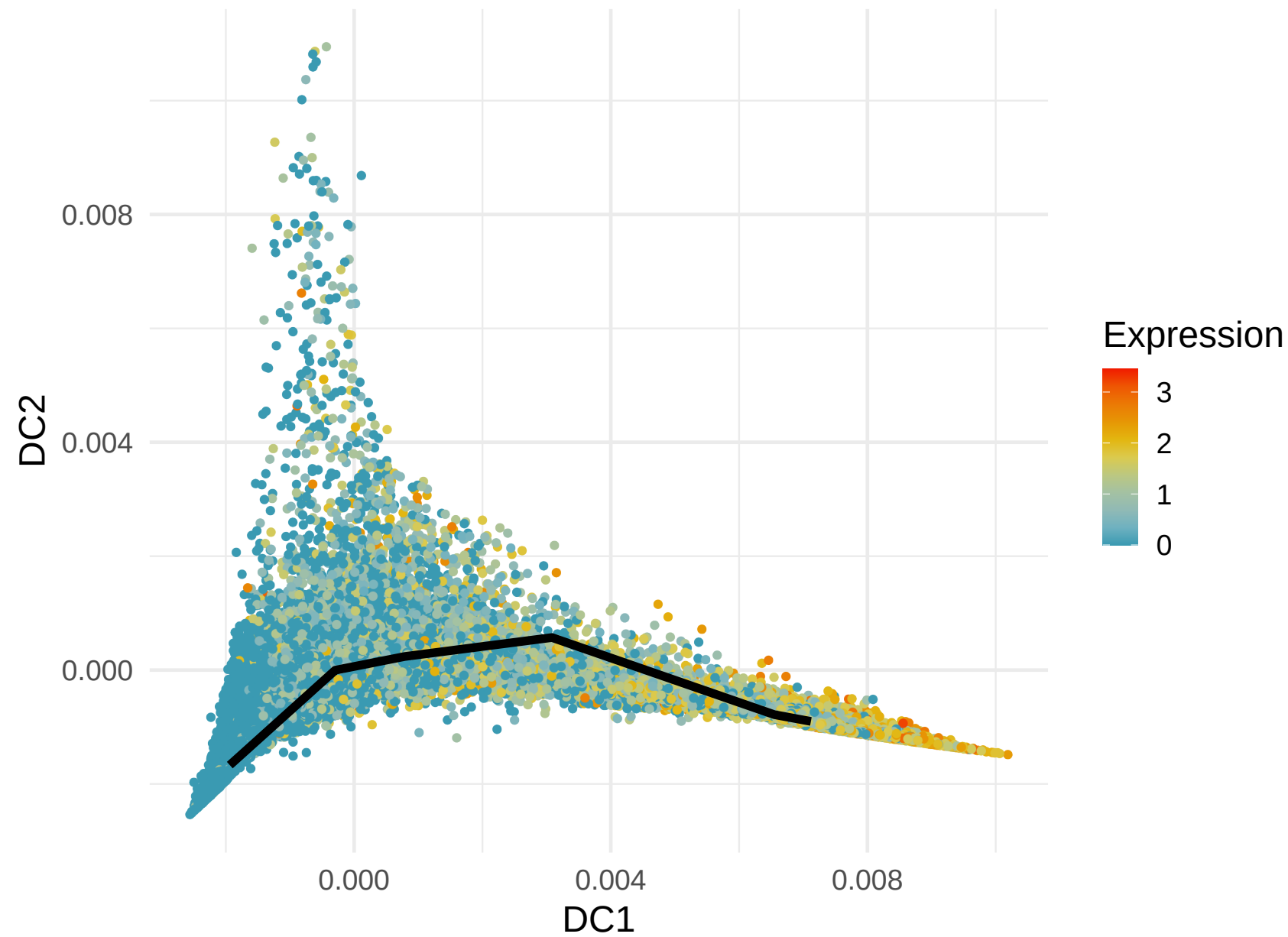
RHOC Expression along Lineage 3 ( R = 0.579 )
