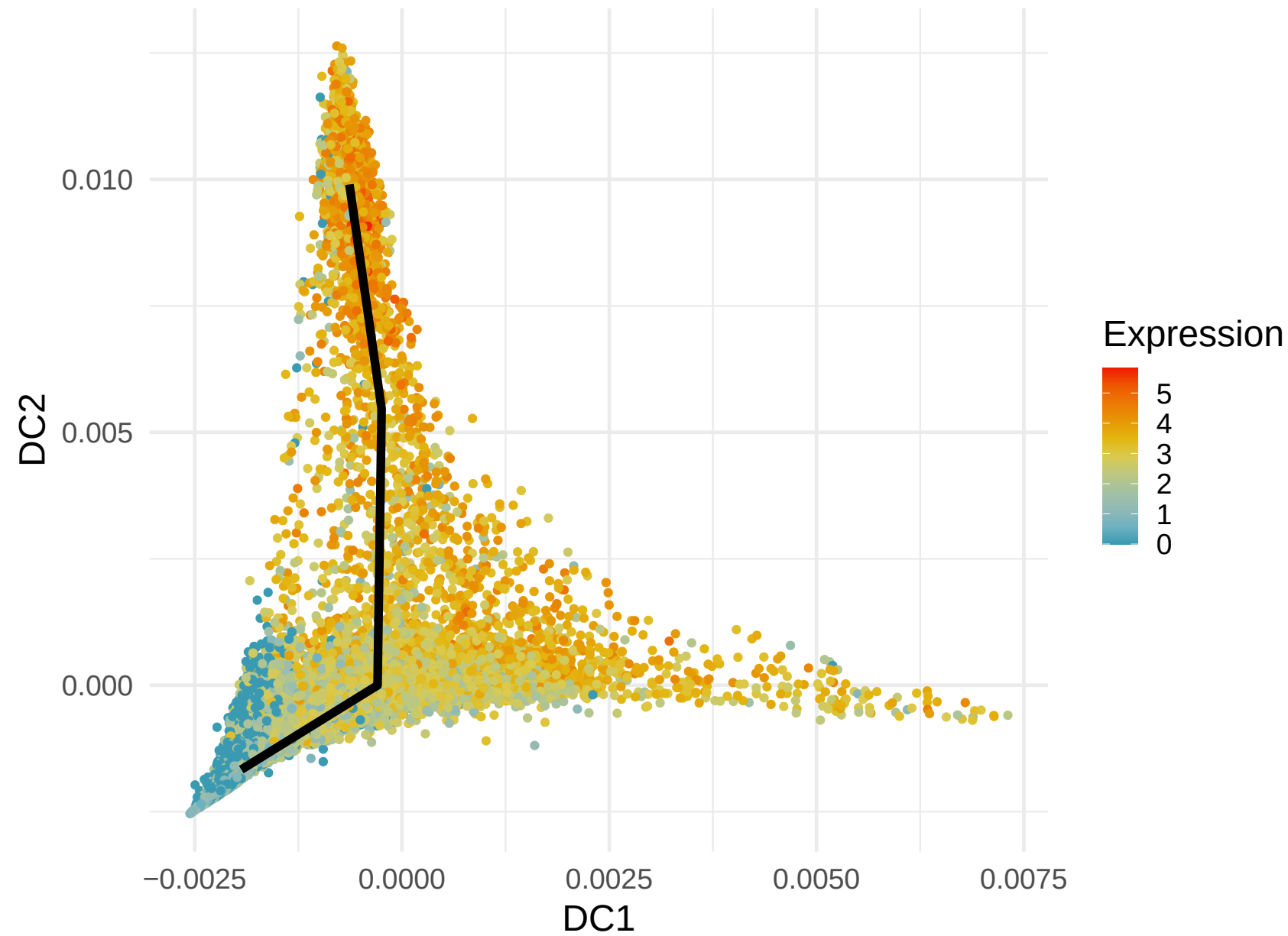
HLA-DRB1 Expression along Lineage 4 ( R = 0.41 )
