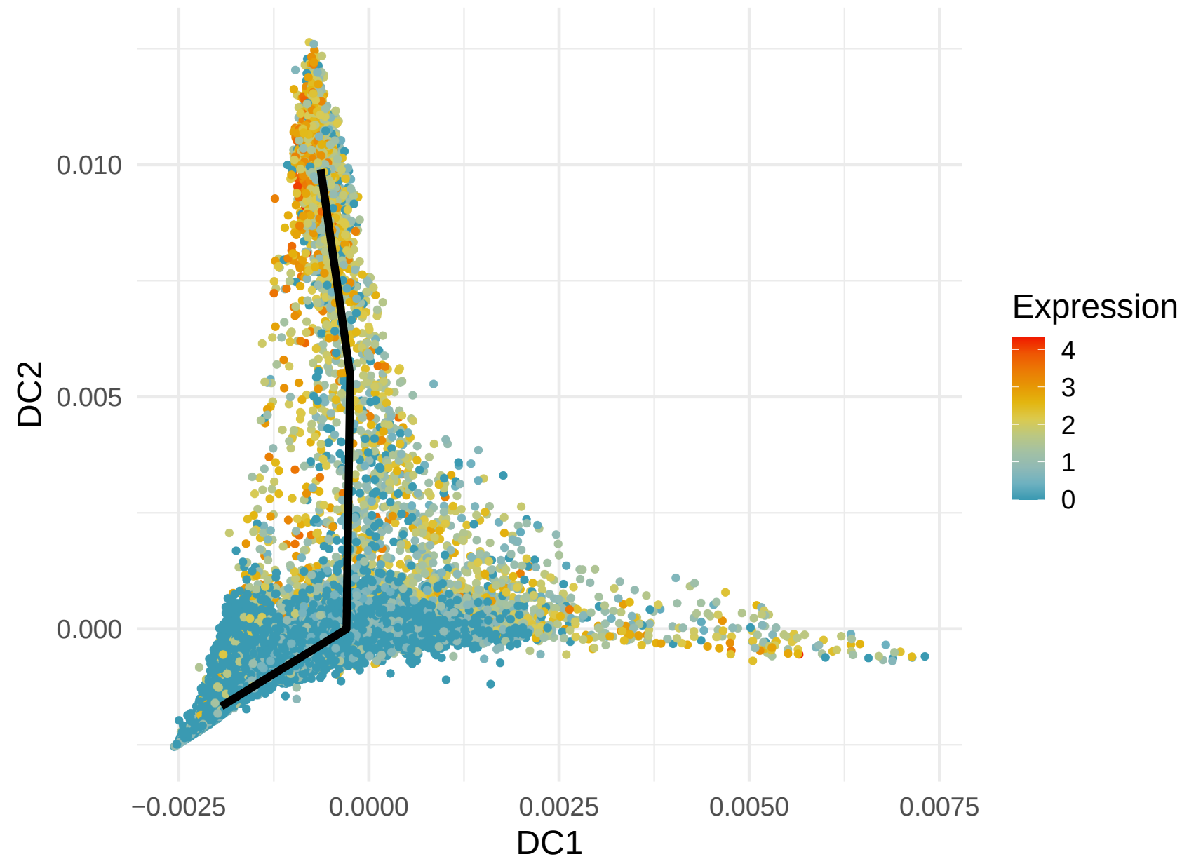
MT-ND6 Expression along Lineage 4 ( R = 0.324 )
