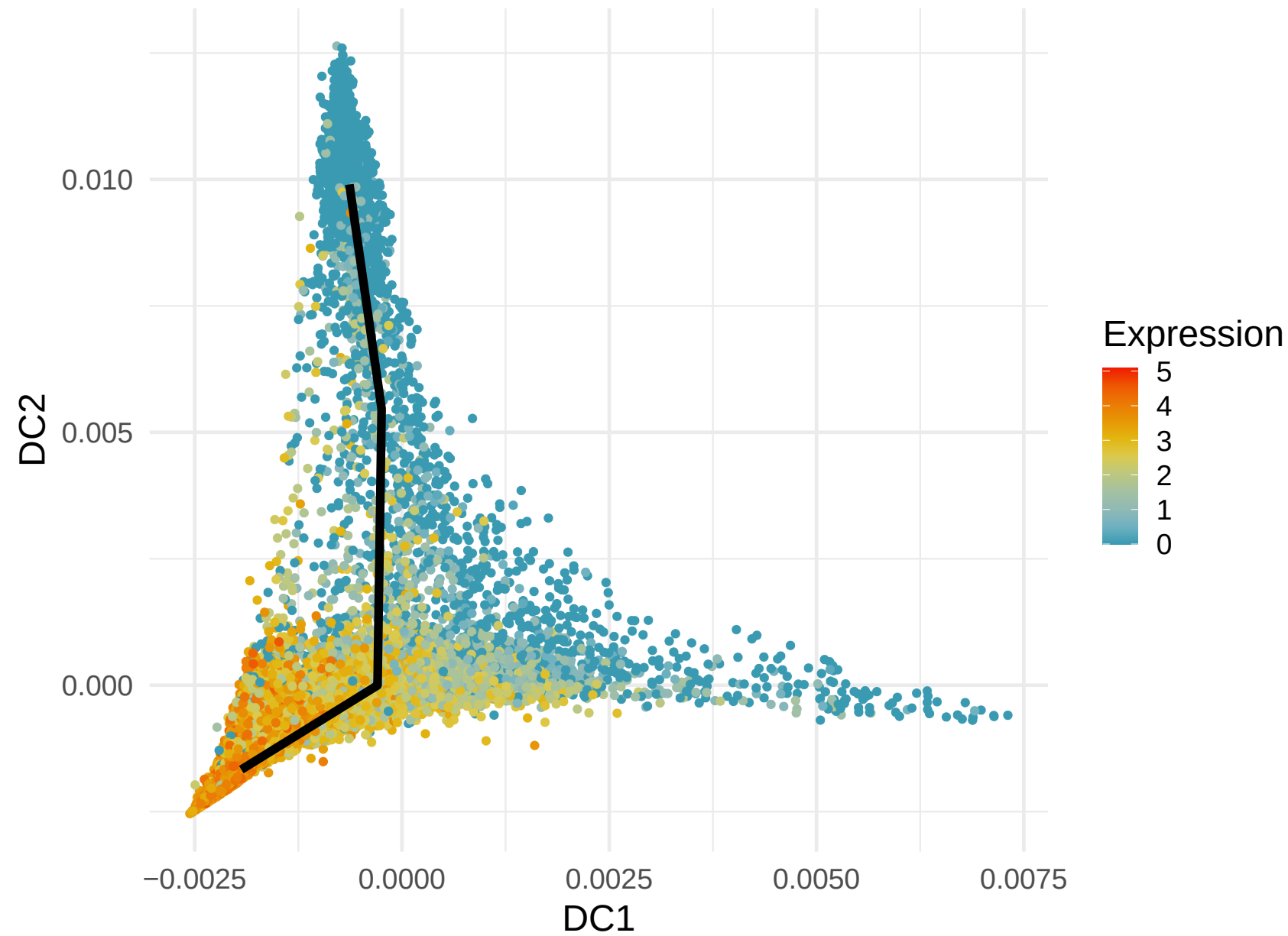
VCAN Expression along Lineage 4 ( R = -0.388 )
