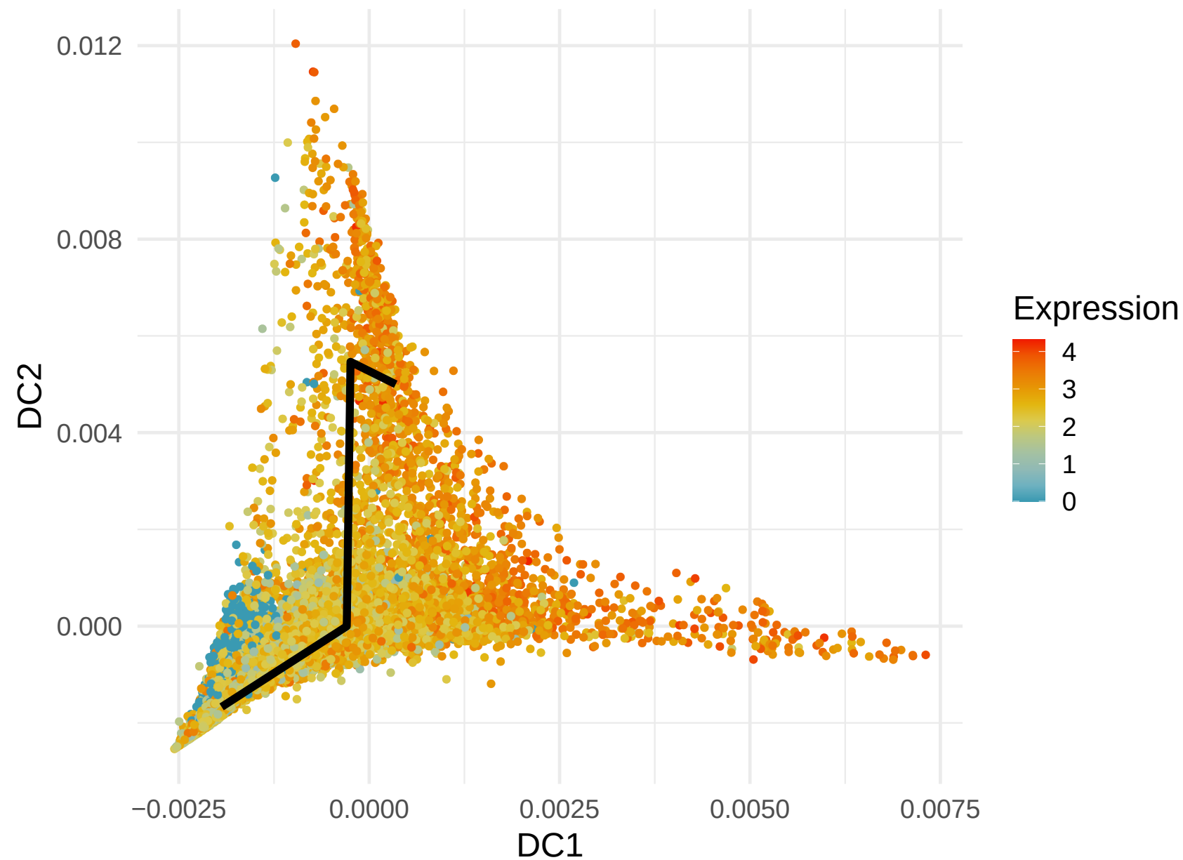
FCER1G Expression along Lineage 6 (R= 0.375)
