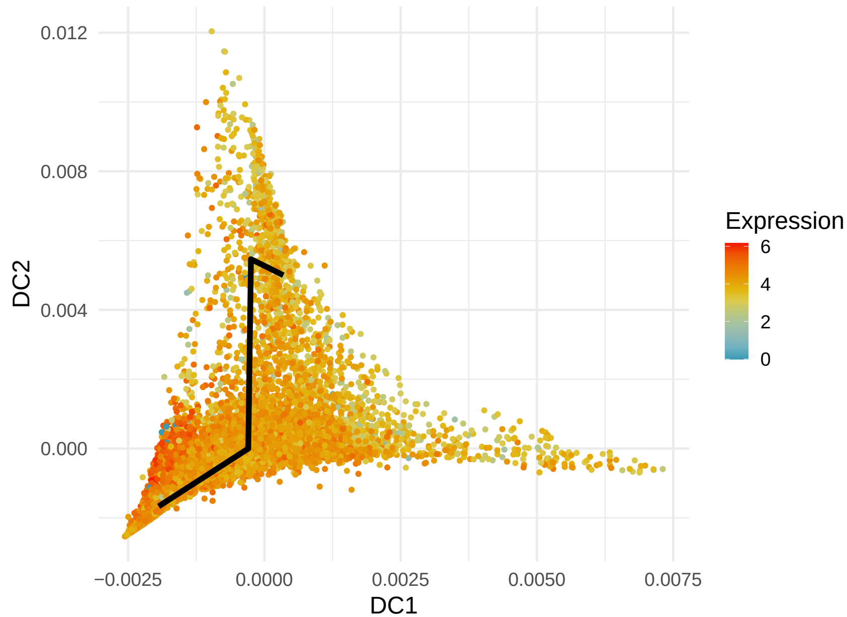
MT-CO 2 Expression along Lineage 6 ( R = -0.405 )
