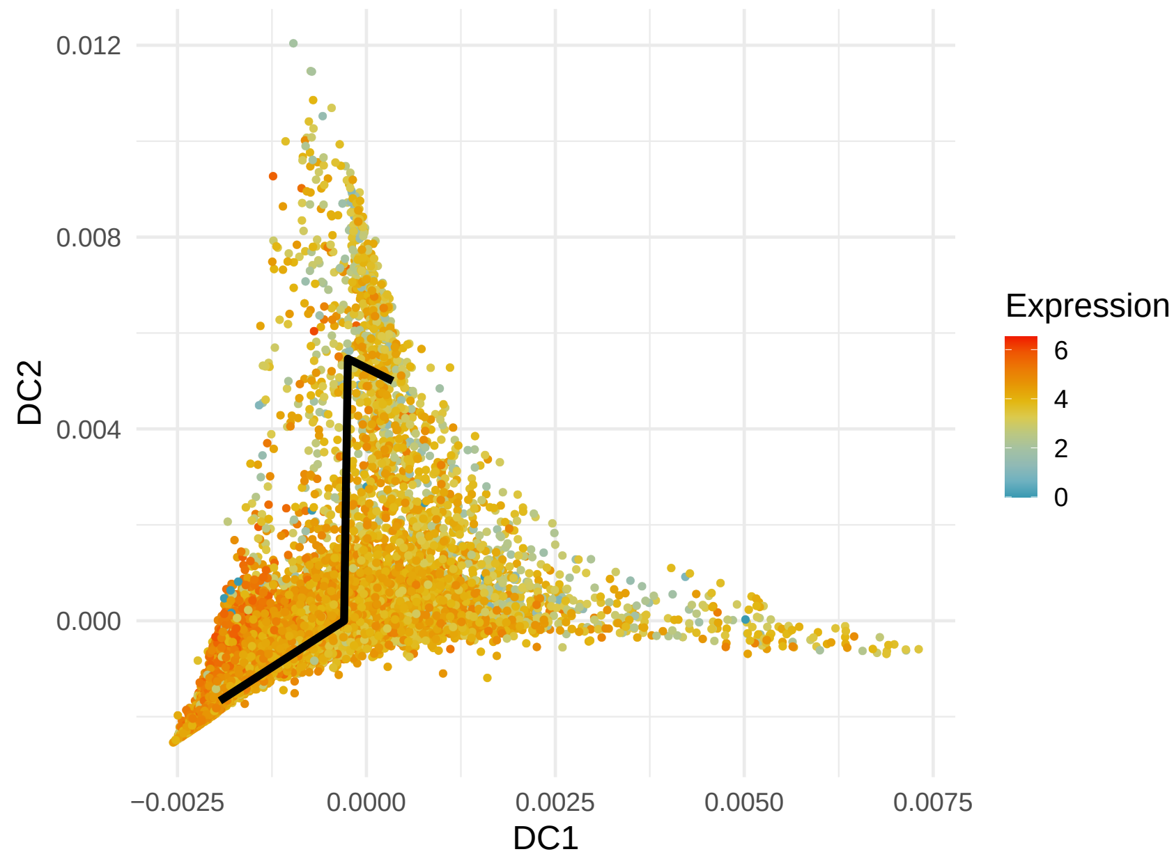
MT-CO3 Expression along Lineage 6 ( R = -0.34 )
