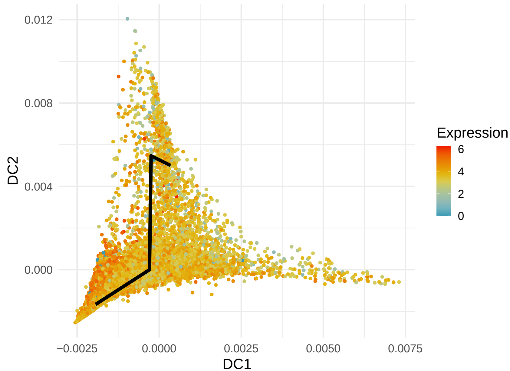
MT-ND3 Expression along Lineage 6 ( R = -0.306 )
