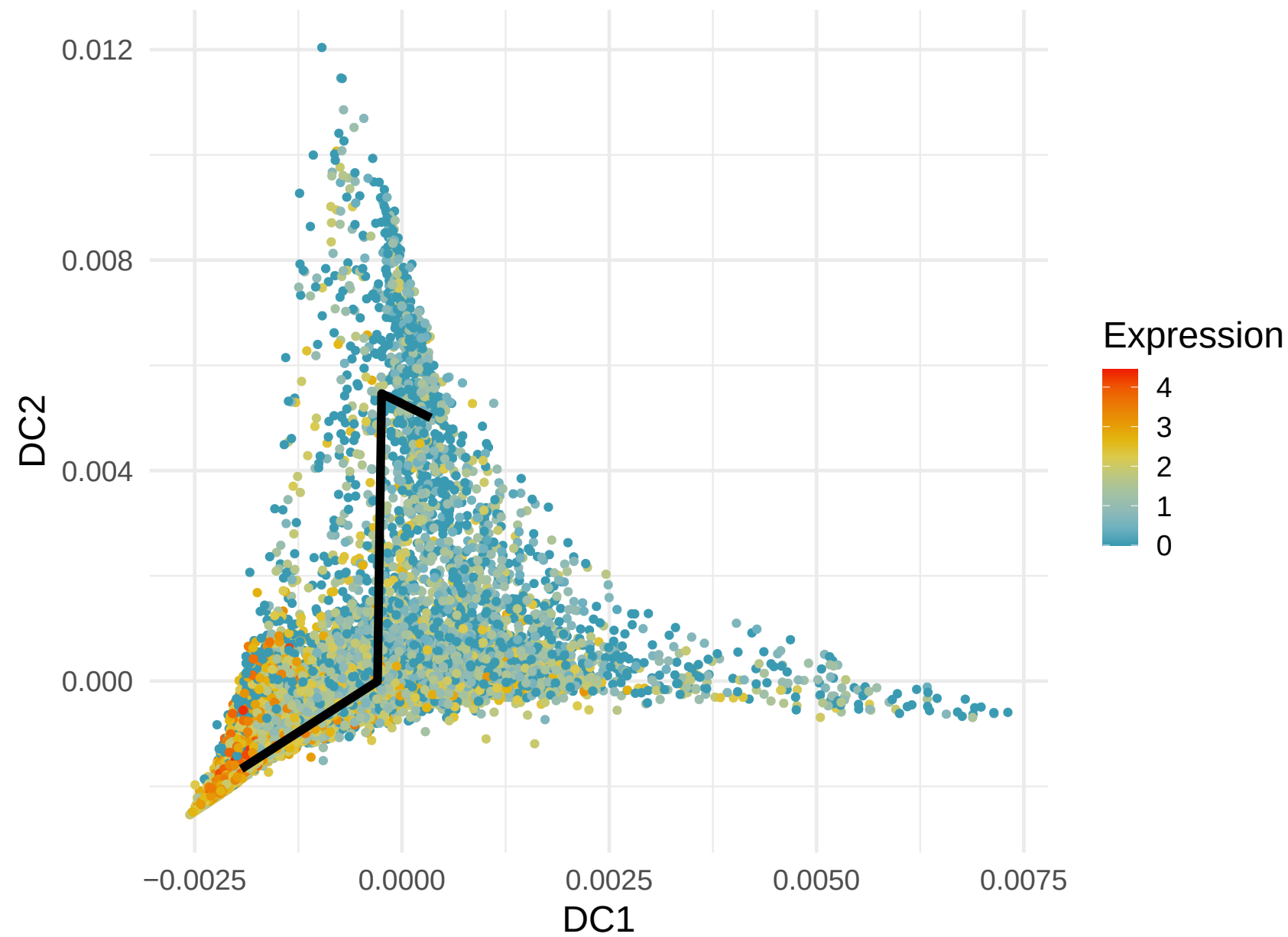
RGS2 Expression along Lineage 6 ( R = -0.292 )
