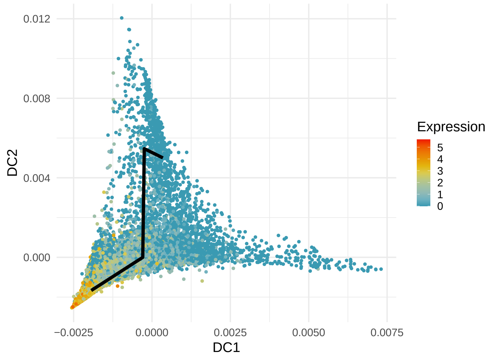
S100A12 Expression along Lineage 6 ( R = -0.339 )
