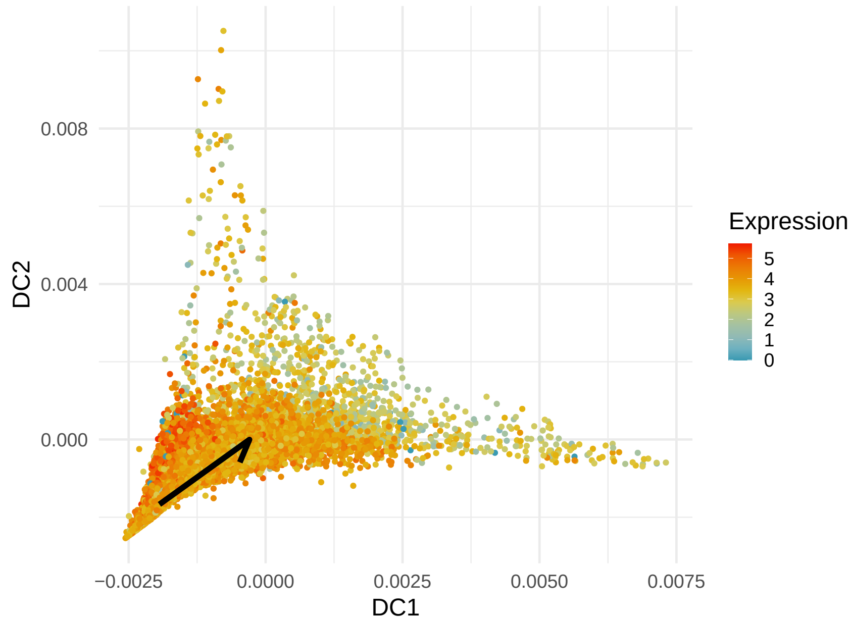
MT-ND1 Expression along Lineage 7 ( R = -0.208 )
