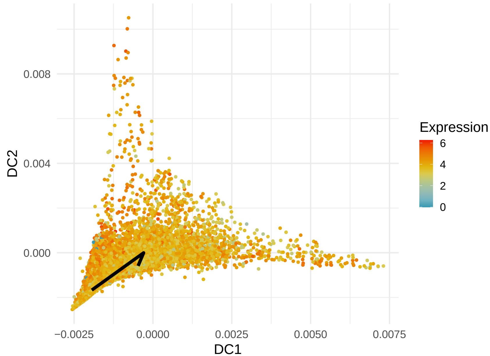
MT-ND4 Expression along Lineage 7 ( R = -0.173 )
