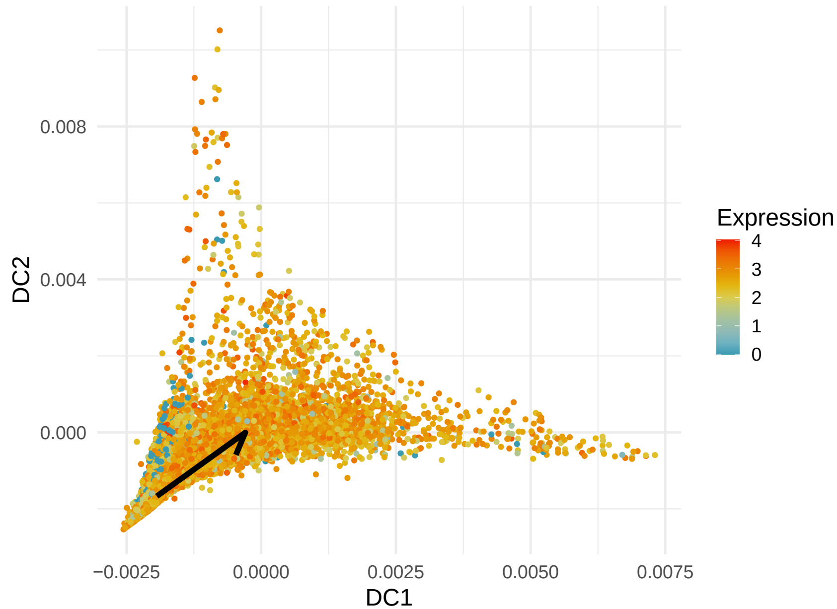
RPL7A Expression along Lineage 7 ( R = 0.38 )
