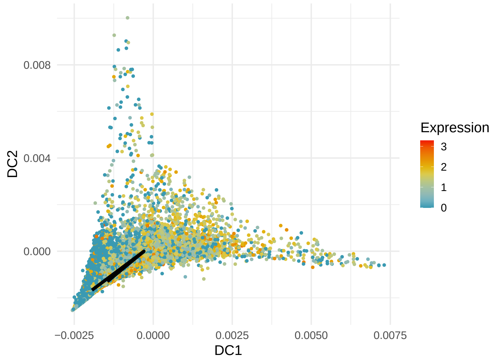
EPSTI1 Expression along Lineage 8 ( R = 0.311 )
