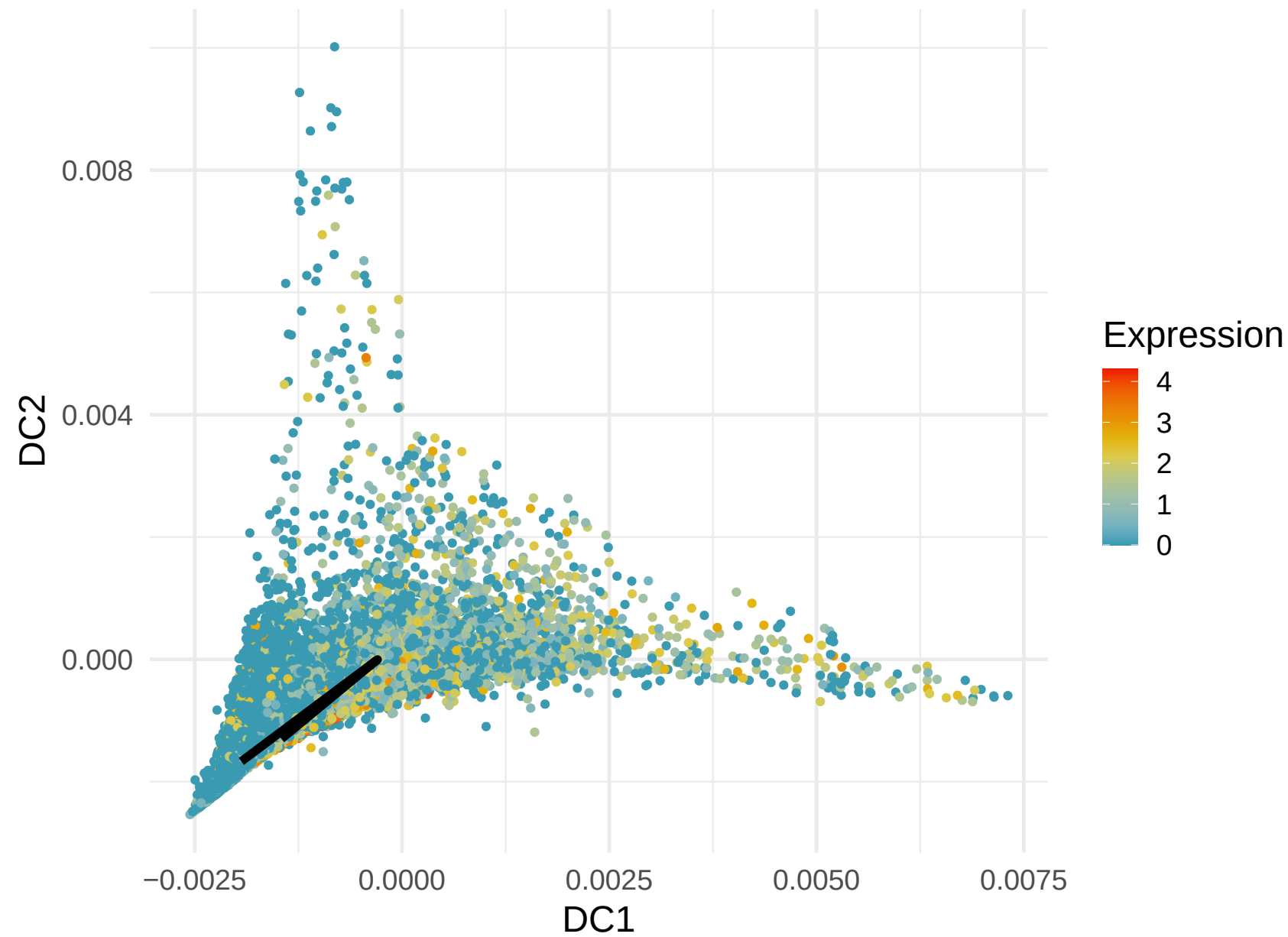
IFIT1 Expression along Lineage 8 (R= 0.301)
