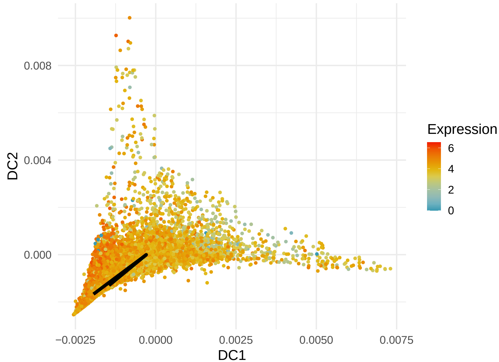
MT-CO3 Expression along Lineage 8 ( R = -0.268 )
