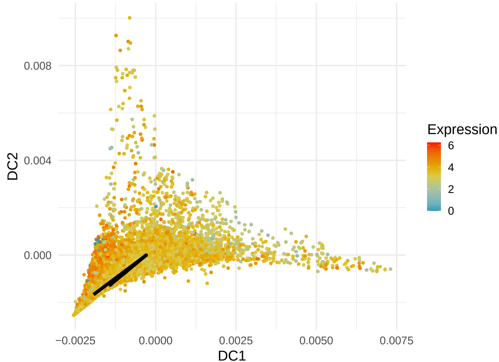
MT-ND2 Expression along Lineage 8 ( R = -0.25 )
